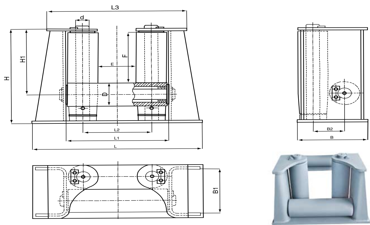
三滚柱导缆器-A Three-roller fairlead-Type A CB*3062-79
