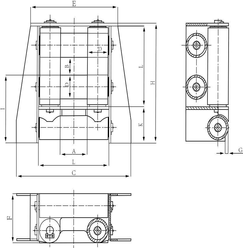
德式五滚柱导缆器 German standard five-roller fairlead
