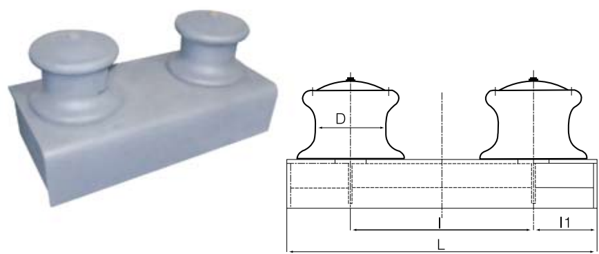
开式二滚轮导缆器 Open type two-roller fairlead
