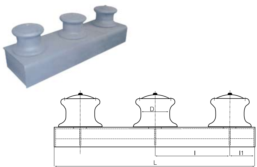
开式三滚轮导缆器 Open type three-roller fairlead
