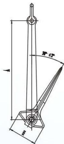
A 型丹福尔锚 DANFORTH HHP. ANCHOR A TYPE
